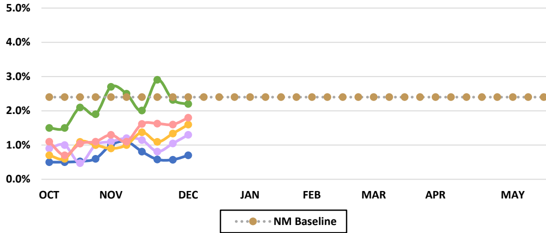
NM ILI Activity by Health Region, 2018-2019
