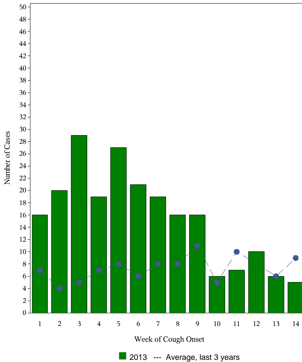
Case Counts of Suspected Pertussis by Week of Cough Onset for 2013
